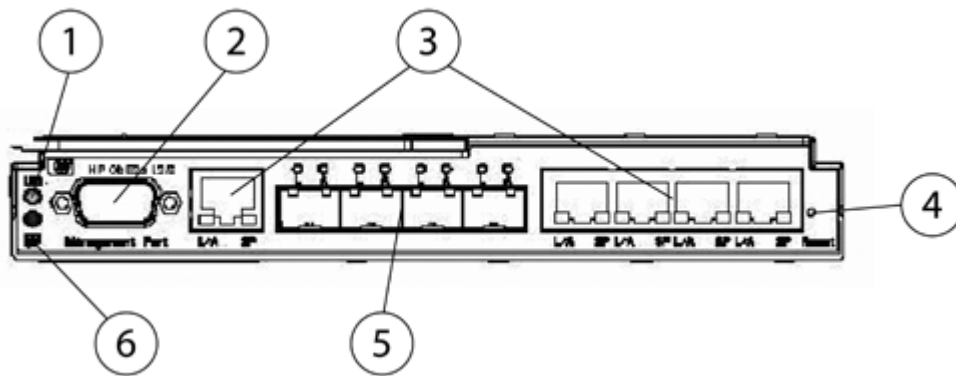
Figure 1 GbE2c Front Bezel
